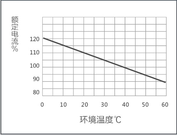
GB800 TM temperature compensation curve
