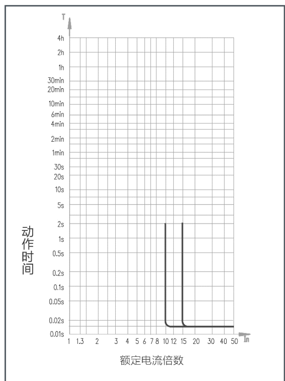
GB400 Time-Current Curves, MC
