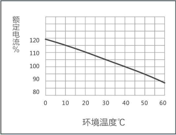
GB400 TM temperature compensation curve
