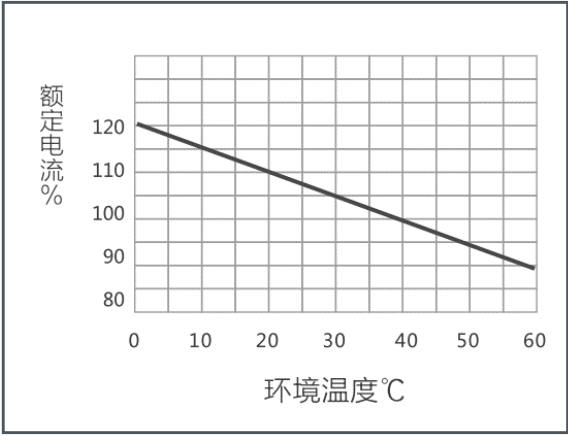
GB630 TM temperature compensation curve
