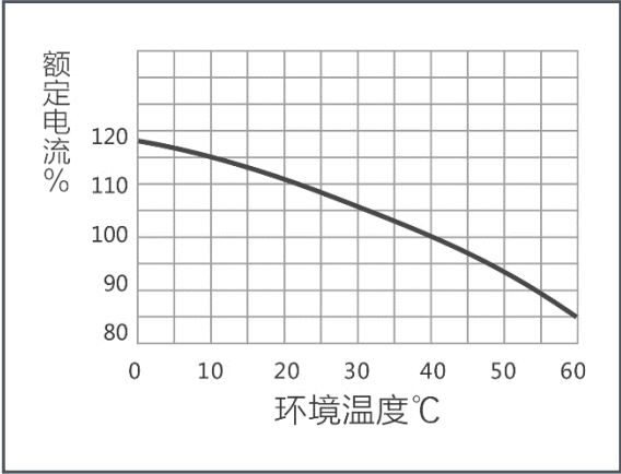
GB250 TM temperature compensation curve
