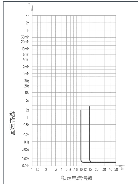
GB250 Time-Current Curves, MC
