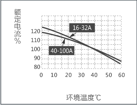
GE100 TM temperature compensation curve
