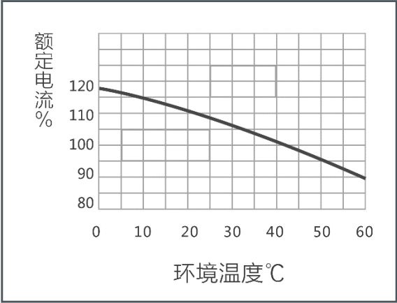
GB160 TM temperature compensation curve
