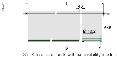
3 or 4 functional units with extensibility module
