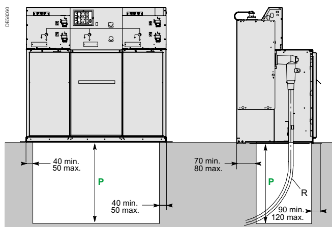
Trench depth P or RM6 without plinth
